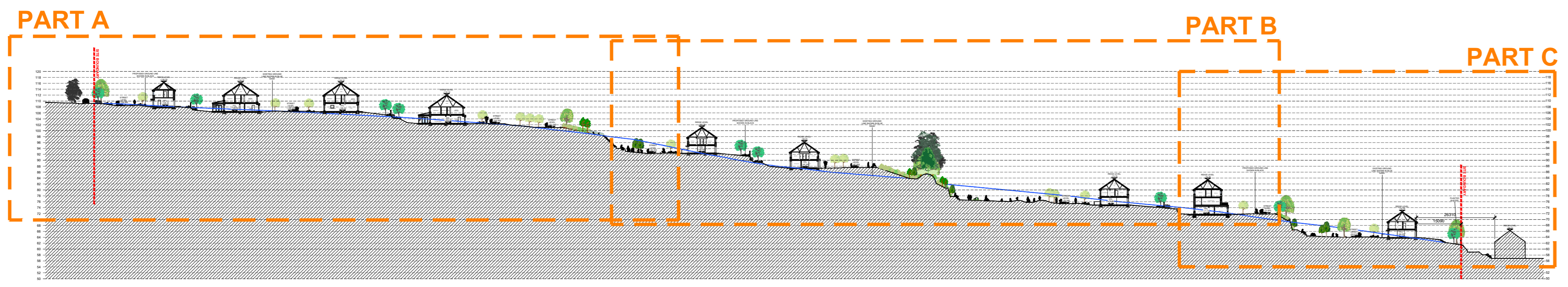
SECTION B-B KEY SCALE 1:1000 @ A0
